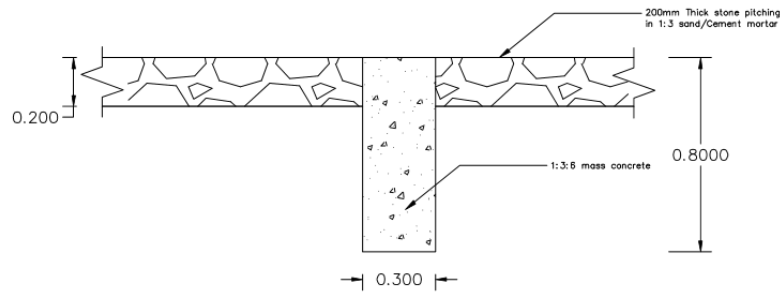
SECTION X-X SPILLWAY CONCRETE SILL (Scale: 1:10)
