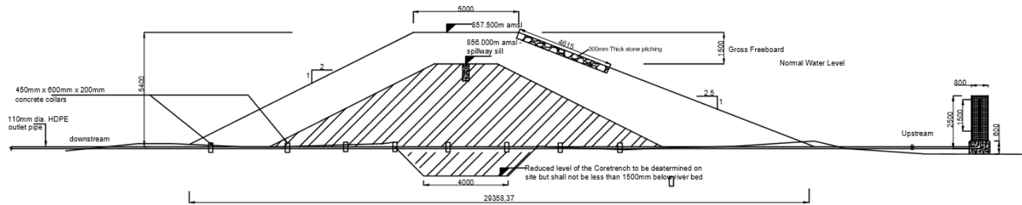
DAM CROSS SECTION AT DEEPEST POINT (Scale: 1:150)
