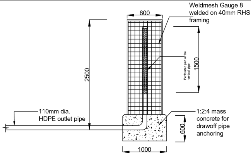
INTAKE TOWER (Scale: 1:30)
